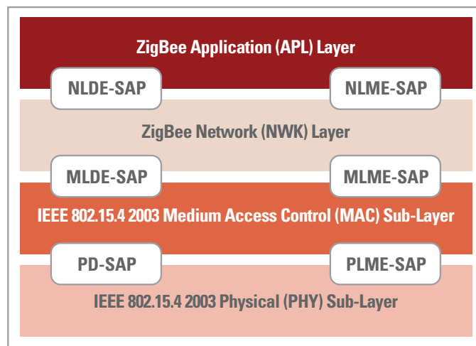
Figure 1 - The ZigBee Stack
