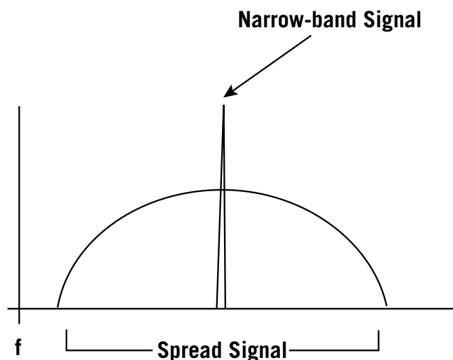
Figure 3 - Spread-Spectrum Signal
