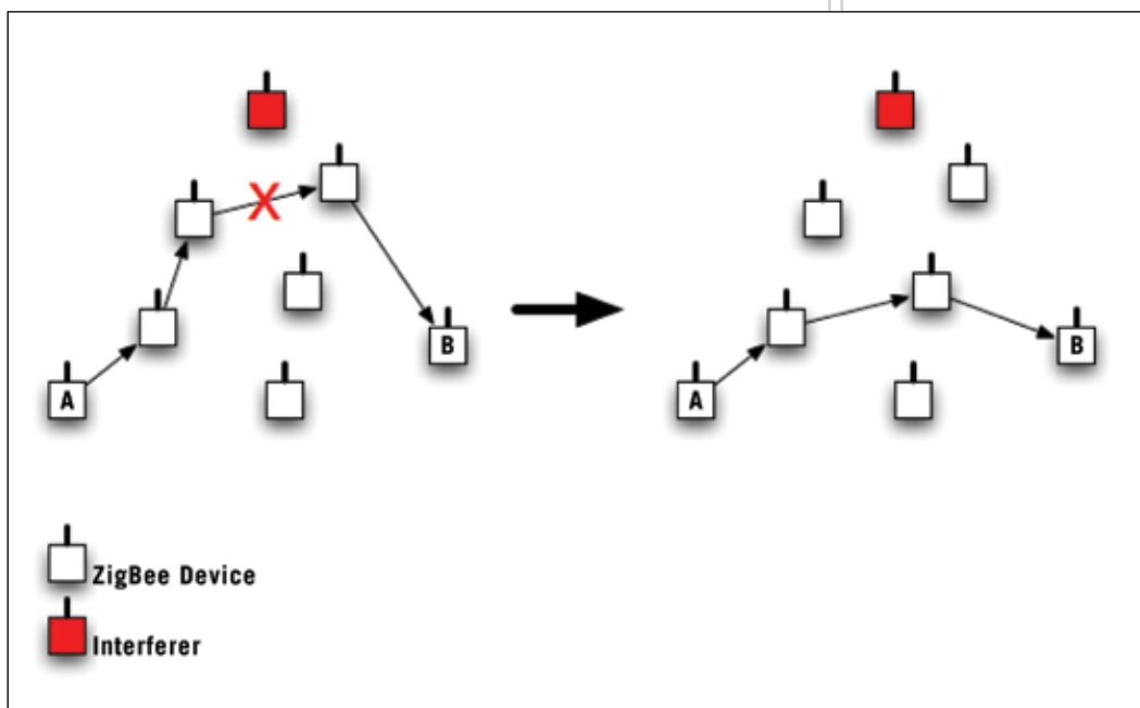
Figure 7 - Mesh Network with Interference
