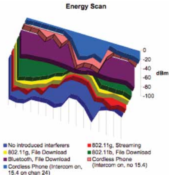
Figure 10 - Interference Sources
