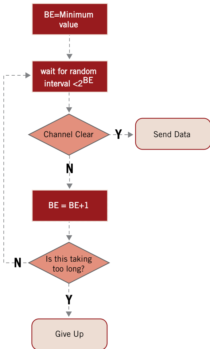
Figure 5 - CSMA
