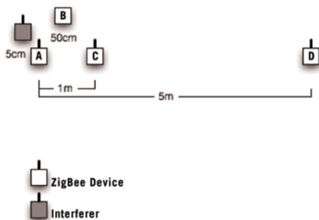
Figure 9 - Test Setup
