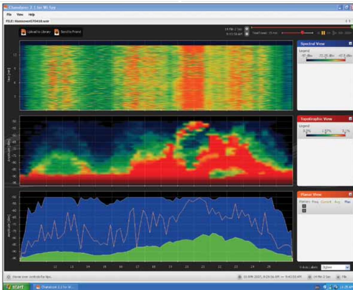
Figure 8 - Hannover Messe Spectrum
