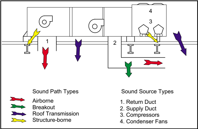
Figure 1: Rooftop unit sound paths.
