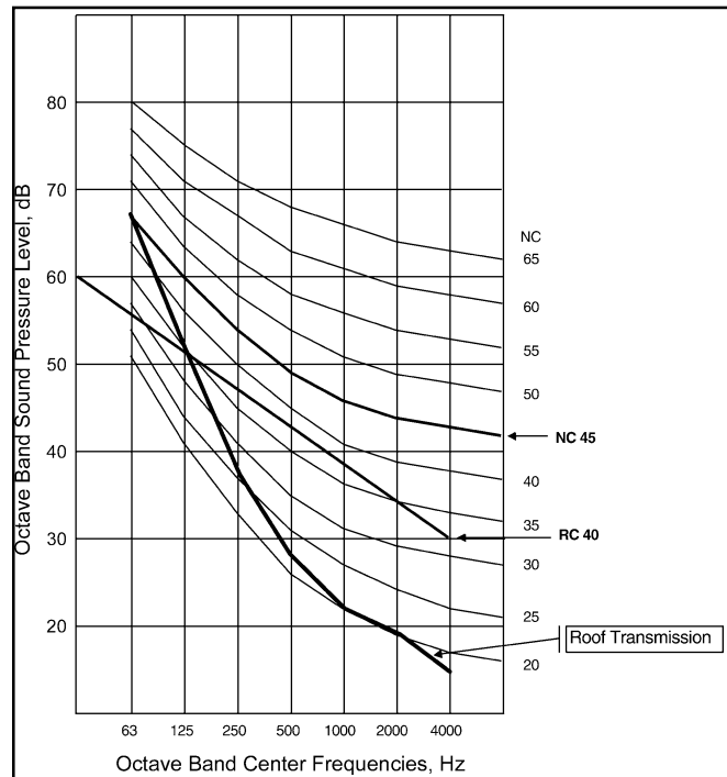
Figure 6: Rooftop unit outdoor noise.
