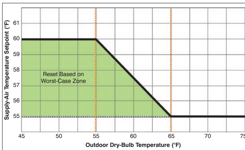
Figure 4: Example of supply-air temperature (SAT) reset control.
