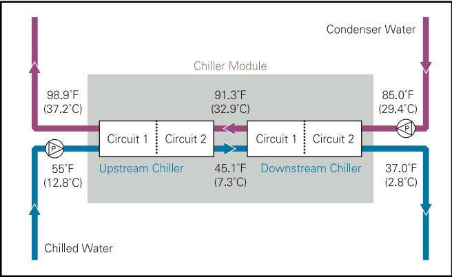
Figure 1: Series–series counterflow arrangement.
