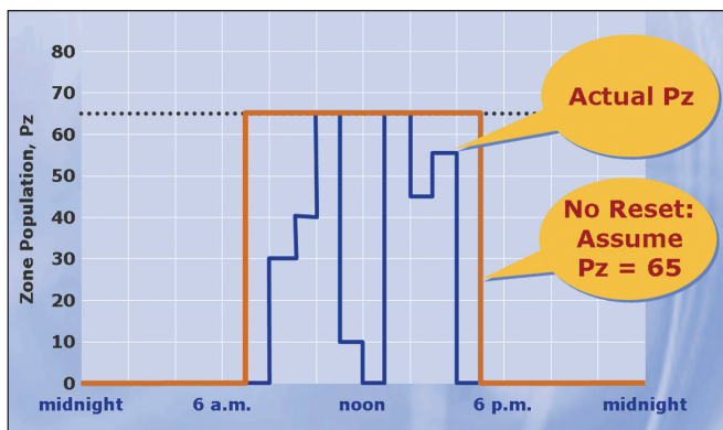
Figure 3 (left): Population profile. Figure 4 (right): Without dynamic reset: OA flow and CO 2 level.
