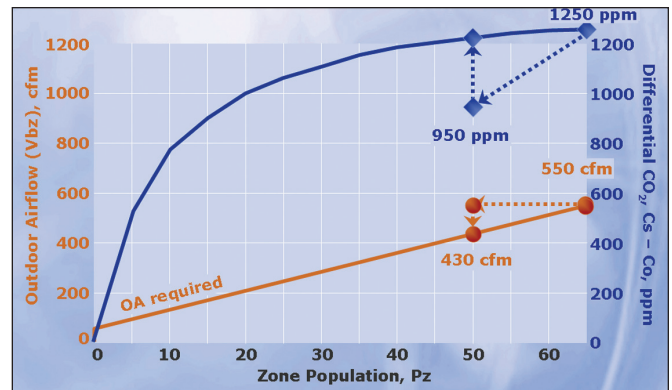
Figure 1 (left): Standard 62-2001: required OA flow and CO 2 level. Figure 2 (right): Standard 62.1-2004: required OA flow and CO 2 level.
