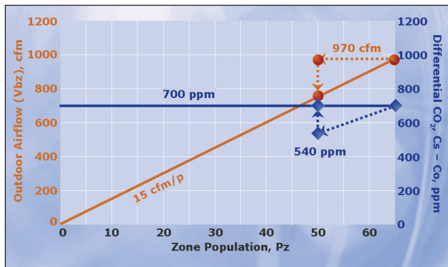
Figure 1 (left): Standard 62-2001: required OA flow and CO 2 level. Figure 2 (right): Standard 62.1-2004: required OA flow and CO 2 level.
