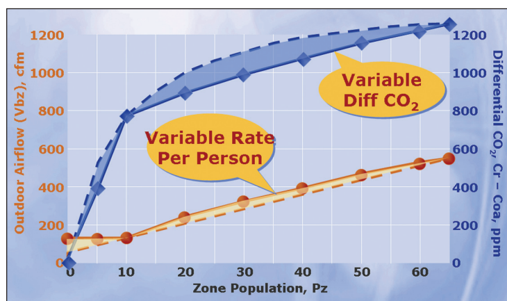
Figure 9: Minimum-to-peak population (modified User's Manual).
