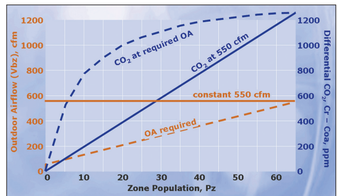
Figure 3 (left): Population profile. Figure 4 (right): Without dynamic reset: OA flow and CO 2 level.
